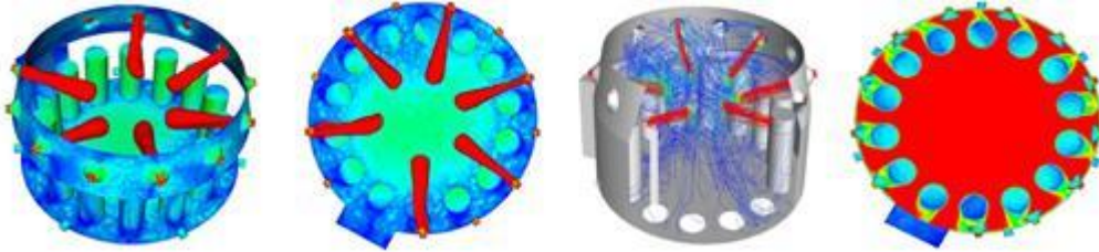
Fig. 1 Detailed CFD analysis was completed to ensure temperature uniformity
